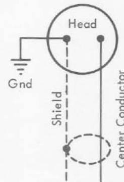
Figure 2 - Wiring Diagram
