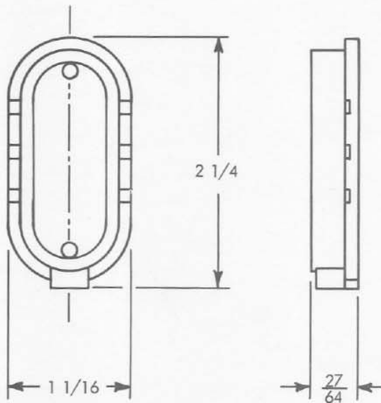
Figure 1 - Dimensions
